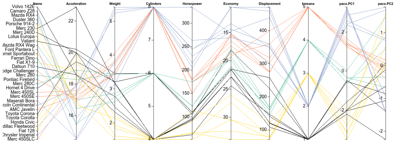
Fig. 1. Parallel coordinates, showing two principal components and a k-means clustering results, both calculated in R. Following the colored patterns we see that in this particular instance the clustering captures the first principal component quite well.
